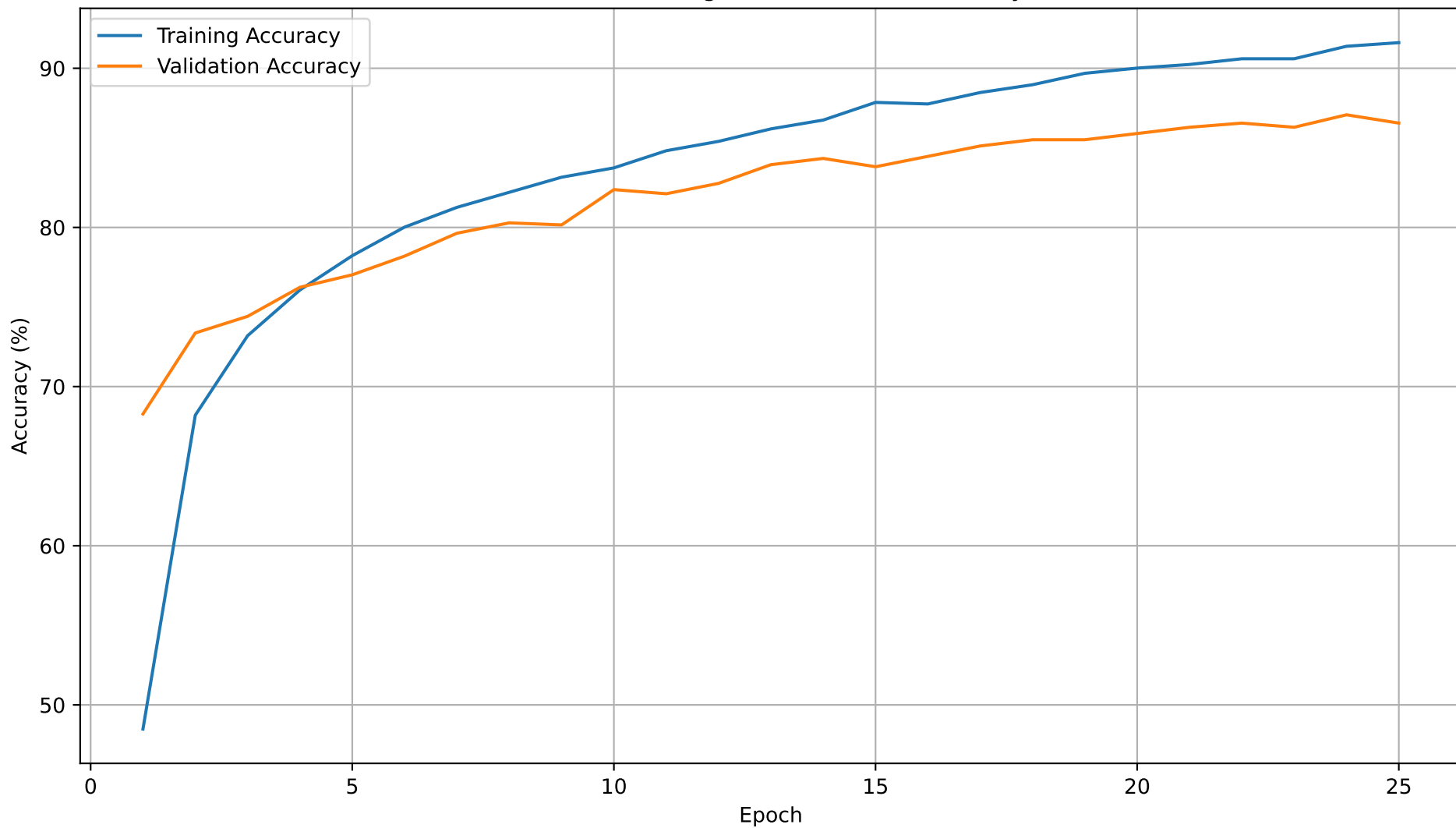
DINOv2 Training and Validation Accuracy
