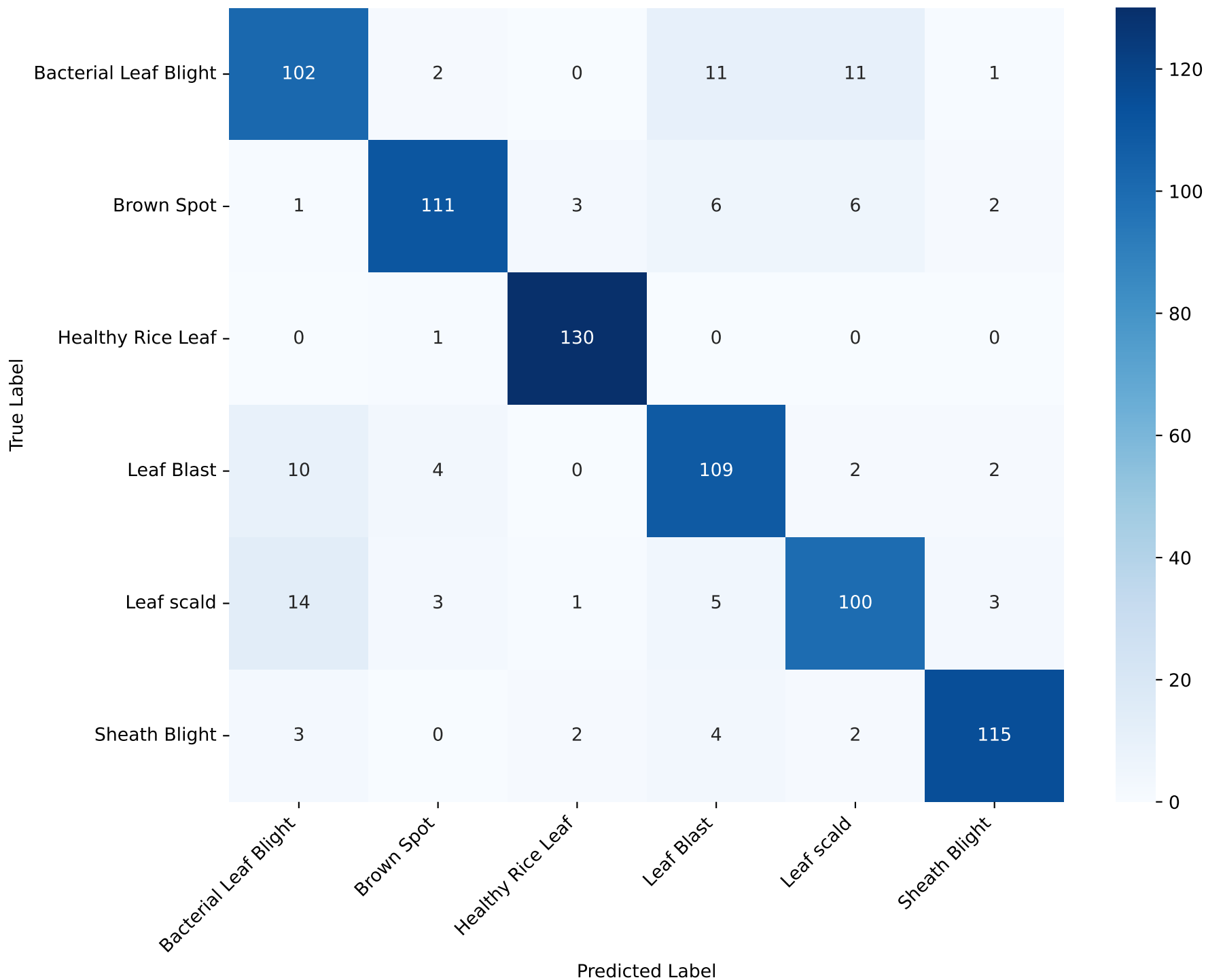
DINOv2 Confusion Matrix
